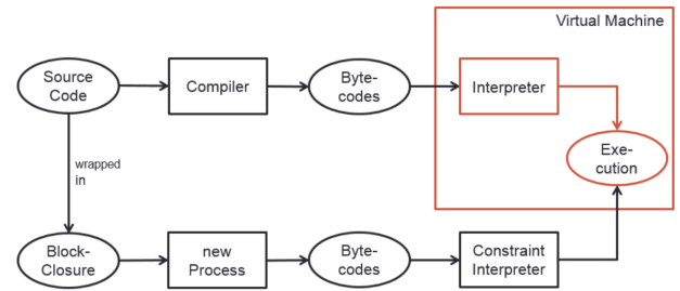
Figure 1: The architecture of Babelsberg/S constraint construction mode
